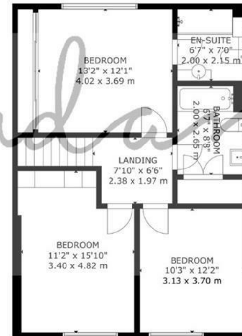
FLOOR 2
